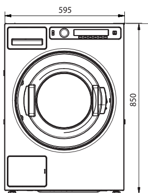
SC70 Front
