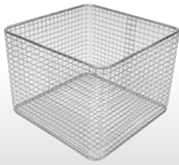
Basket with wire mesh 8 x 8 x 1 mm. Dimensions: 200 x 200 x 150 mm. ref. 8300138
