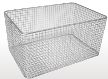
Basket with wire mesh 8 x 8 x 1 mm. Dimensions: 300 x 200 x 150 mm. ref. 8300143
