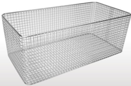
Basket with wire mesh 8 x 8 x 1 mm. Dimensions: 400 x 200 x 150 mm. ref. 8300145
